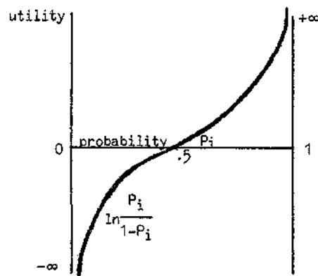
Fig. 1. Transformation of the individual utility function (defined at the range [-\infty; +\infty] ) to the probability P_i (defined at the interval [0;1] ) by means of the so-called logit, specified as: \ln[P_i/(1-P_i)] .
