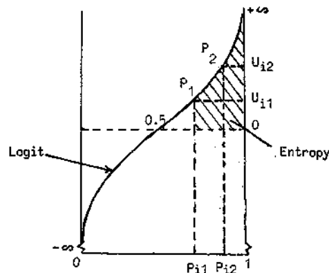
Fig. 2. Graphical description of the relationship between entropy and logit. Here, u_{11} , is the expression of the value (or utility) of the vector of variables characterizing a given alternative 1, with respect to the choice
